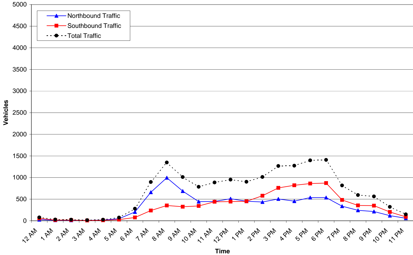
Daily Traffic Volumes - May 27, 2004 Walgrove Avenue - South of Rose Avenue
